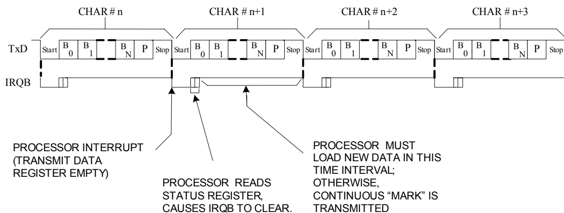
Figure 5 Continuous Data Transmit
