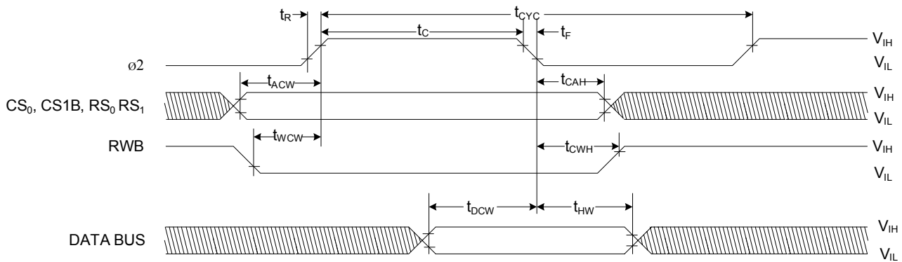
Figure 23 Write Timing Diagram
