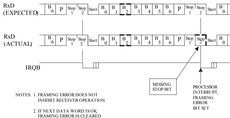
Figure 13 Framing Error
