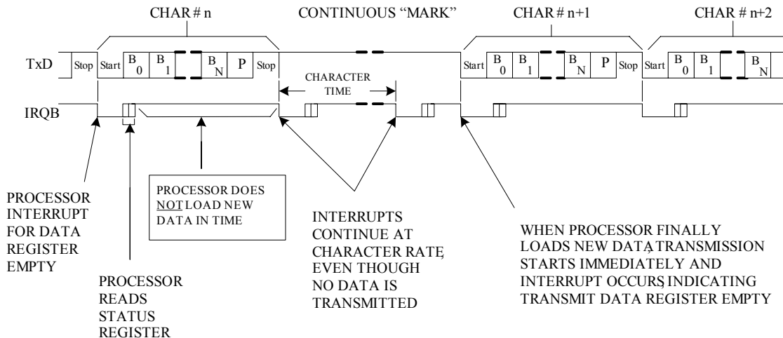
Figure 7 Transmit Data Register Not Loaded by Processor
