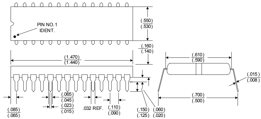
Figure 25 28 Pin Plastic Dip Package Dimensions
