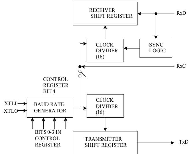
Figure 3 Transmitter/Receiver Clock Circuits
