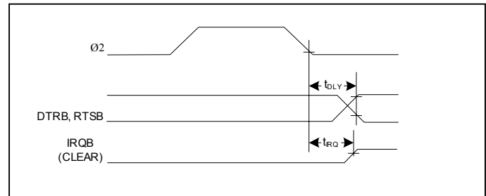
Figure 22 Interrupt and Output Timing
