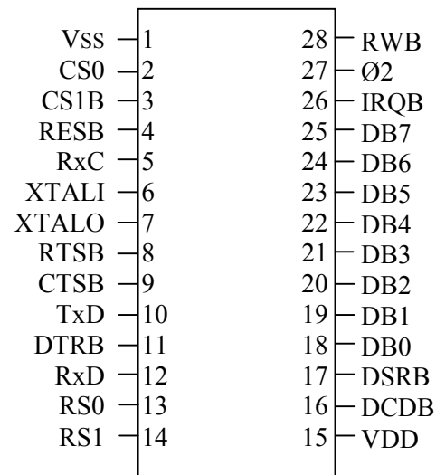
Figure 1 W65C51S ACIA Pin Configuration
