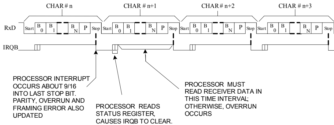
Figure 6 Continuous Data Receive
