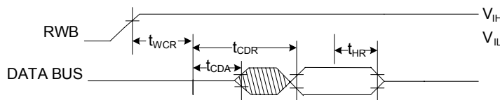
Figure 24 Read Timing Characteristics
