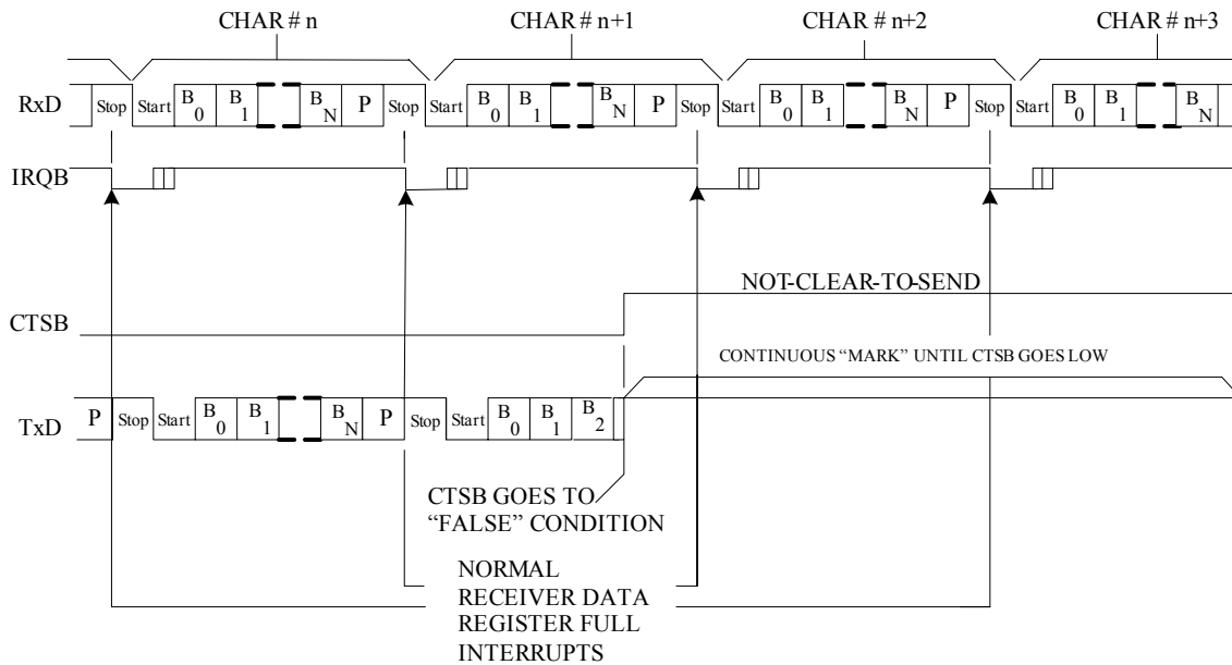
Figure 11 Effect of CTSB on Echo Mode
