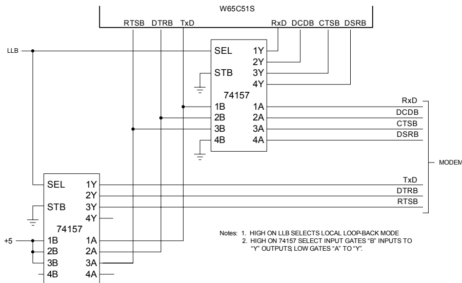
Figure 19 Loop-Back Circuit Schematic
