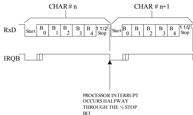
Figure 15 Timing with 1/2 Stop Bits
