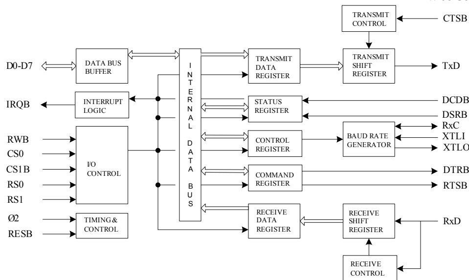
Figure 2 ACIA Internal Organization
